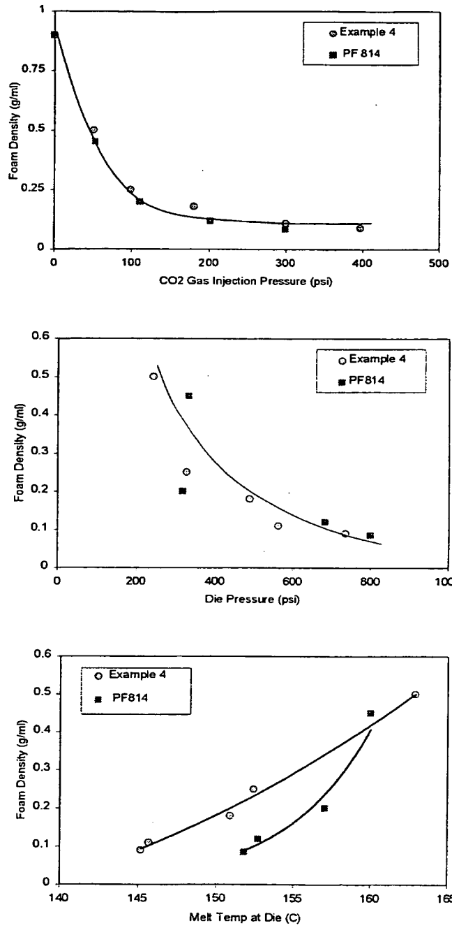
Figure 10: Ex 4 and PF-814 foam processing data for CO 2 gas injection
